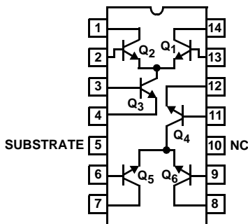
CA3054 (SOIC) TOP VIEW
